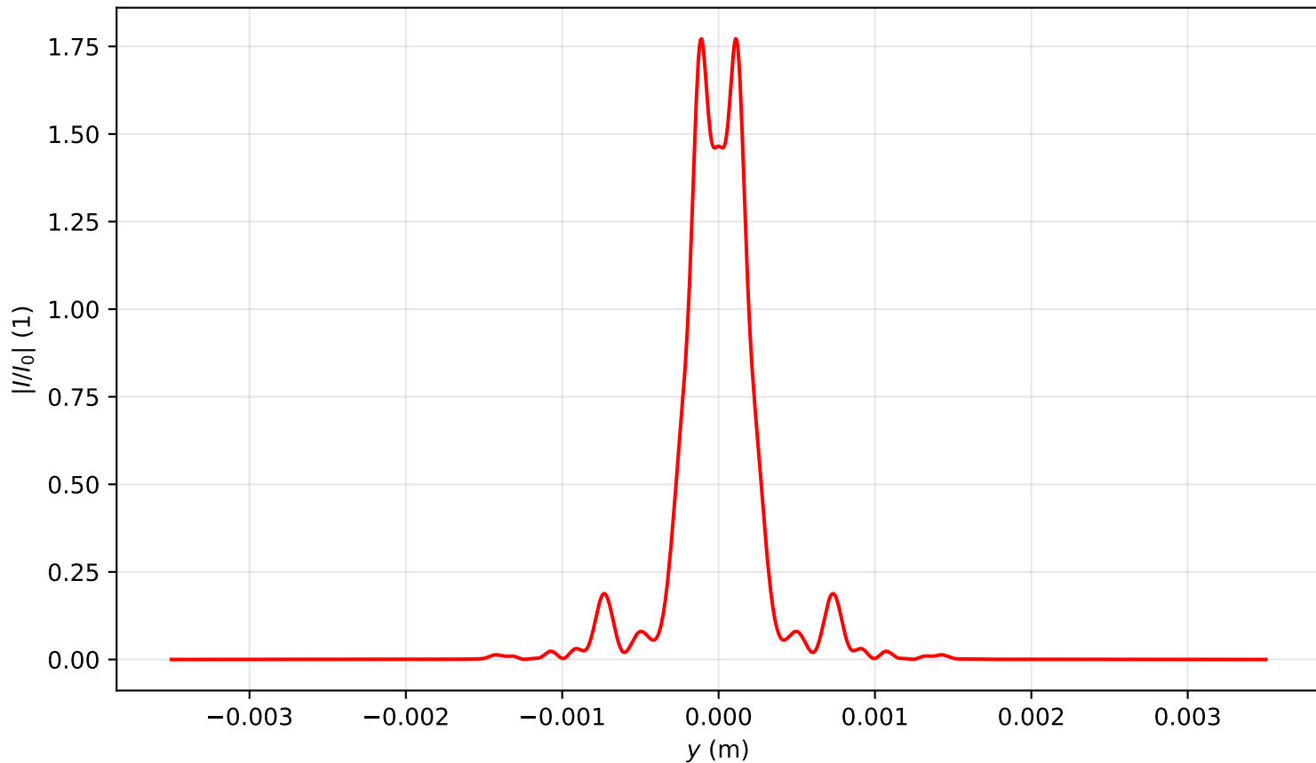
Intensity profile I(x=0, y, z=0.955)/I_0 , \text{Pin}=7.5\text{Pcr} , artificial time
